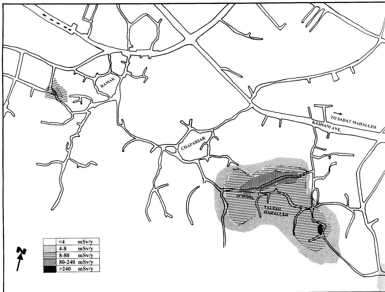
Fig. 2. A map of the HBRA in Ramsar. The areas of highest background are found in discrete locations, corresponding to specific geologic features. Other areas of elevated background radiation levels are found elsewhere in the city; these are the highest levels found in residential areas. Although the locations of individual houses are not noted on this map, the entire area is residential, and 1–2 family houses are spaced about 20–30 m apart along each of the roads shown. On this map, one inch is equal to a distance of about 100 m.
