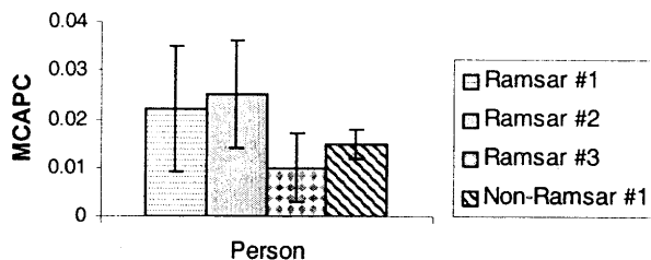
Fig. 4. MCAPC among individuals who live in the Ramsar HBRA and the average of 14 from a nearby control area. Persons 1 and 2 are married and live in a house with radiation levels of about 20 \mu\text{Gy h}^{-1} in the bedroom, giving an average annual radiation dose of 58.4 \text{ mGy y}^{-1} simply from sleeping. Person 3 has a hot spring in her house with radiation levels of up to 50 \mu\text{Gy h}^{-1} . Each data point is based on analysis of 200 cells per person obtained during two separate sampling events. Note that, as in Fig. 1, the 95% confidence intervals all overlap, suggesting that the number of background chromosome abnormalities in these people are statistically similar.
